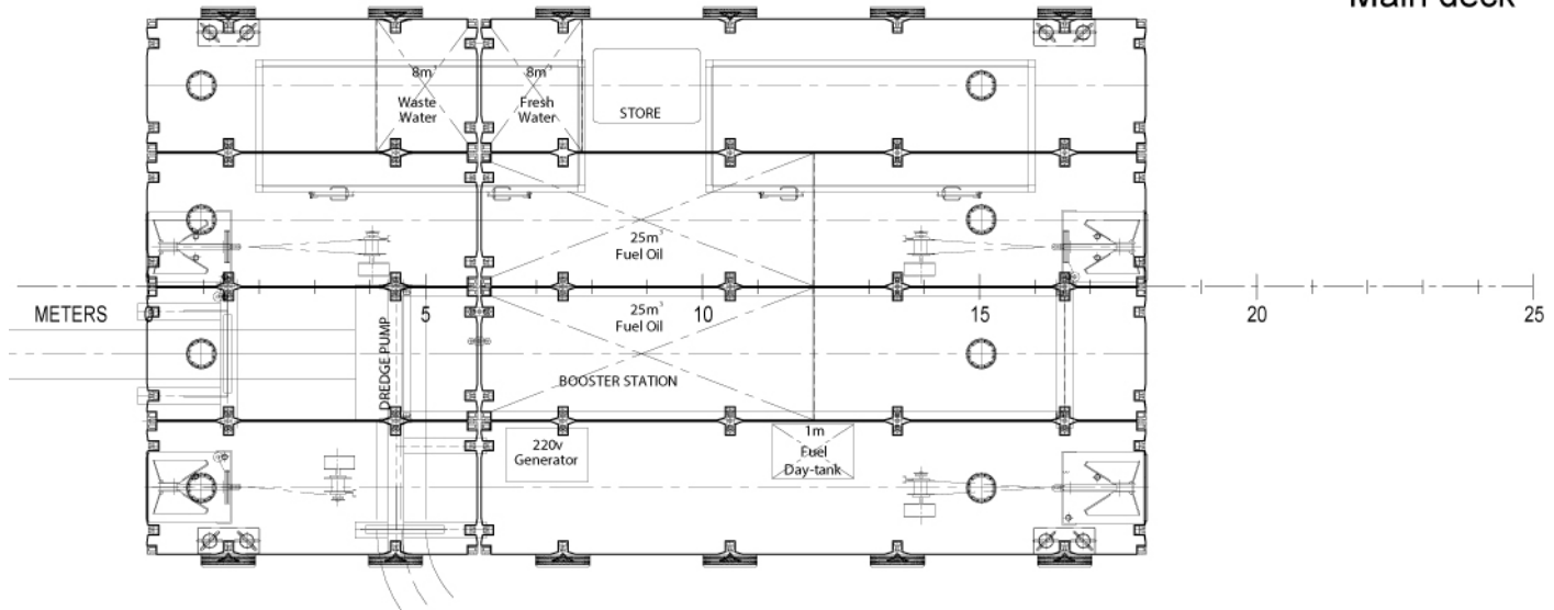
Main deck
