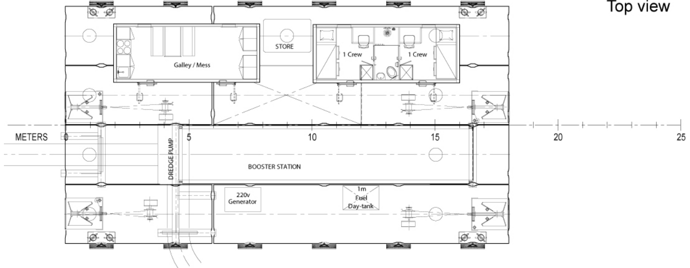
Main deck
