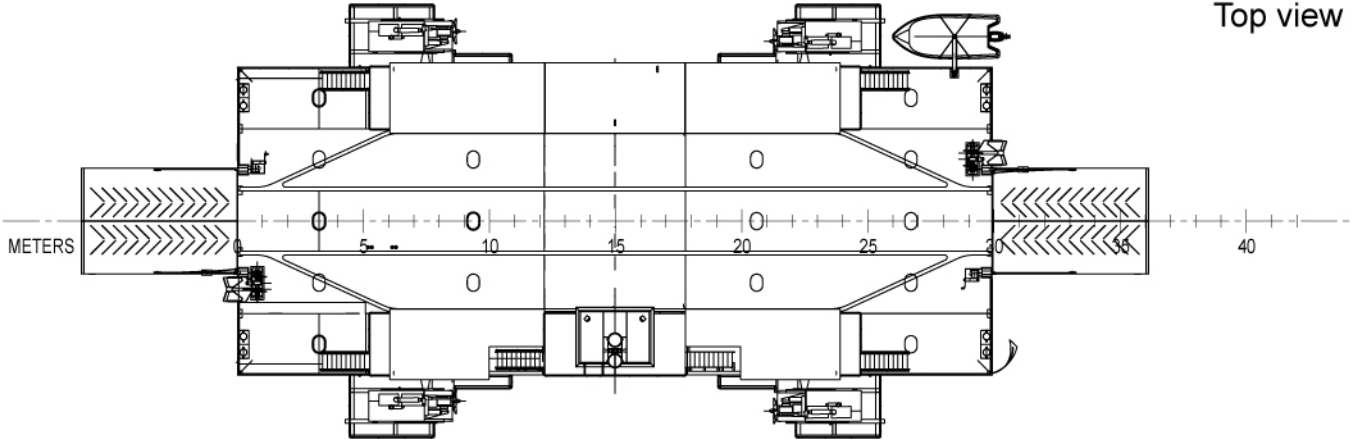
First deck
