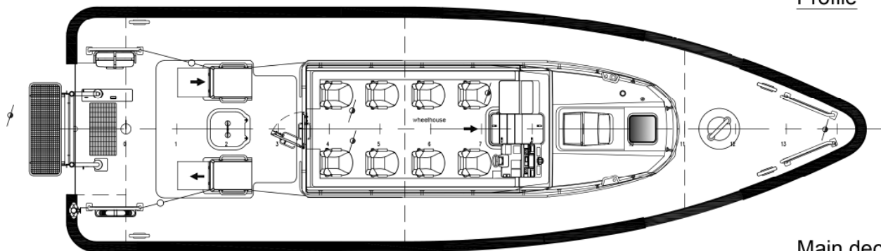
Main deck
