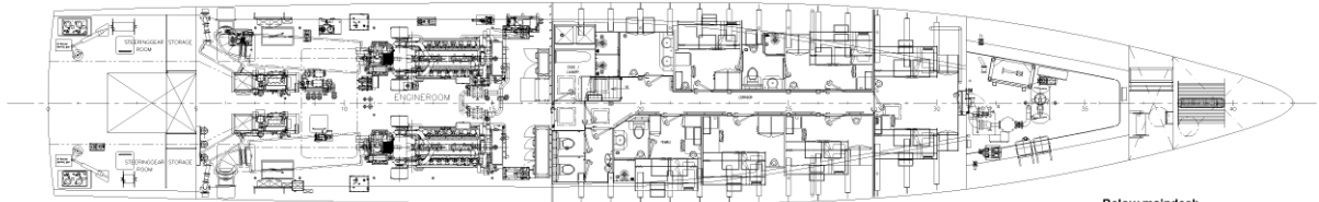
Below maindeck
