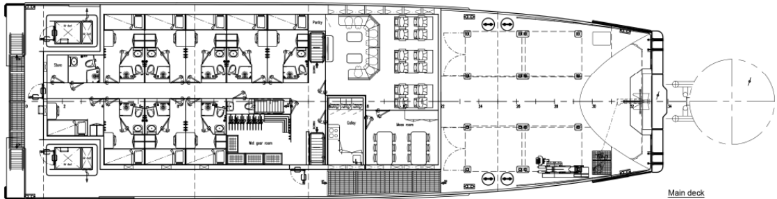
Main deck
