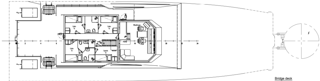
Bridge deck
