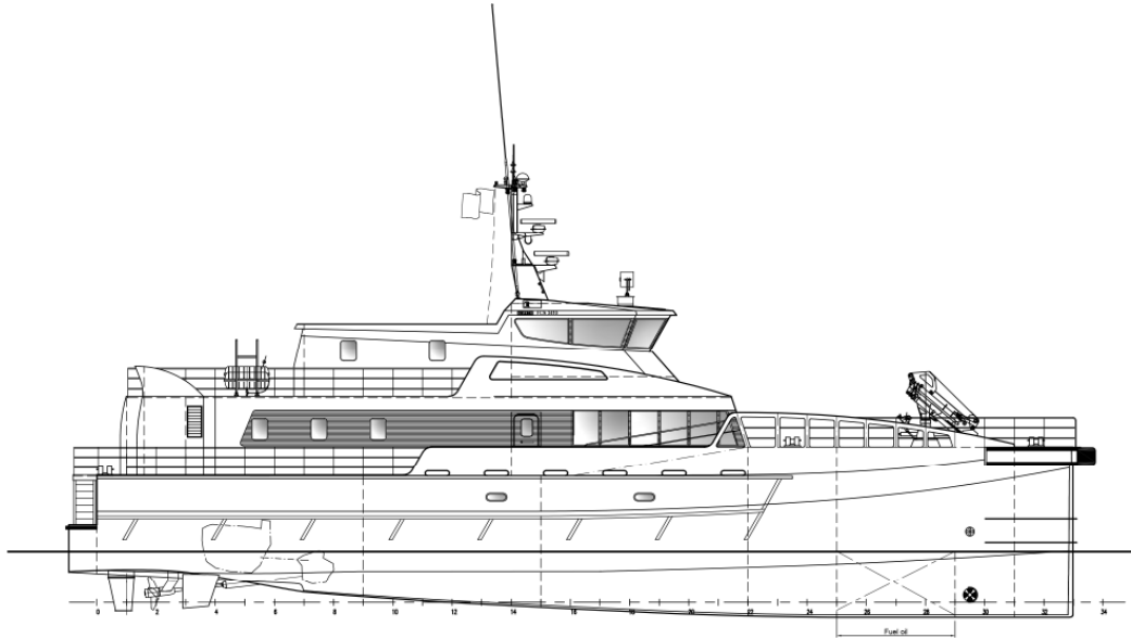
Profile
