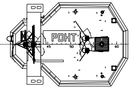
Top deck
