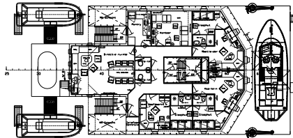
Accommodation deck
